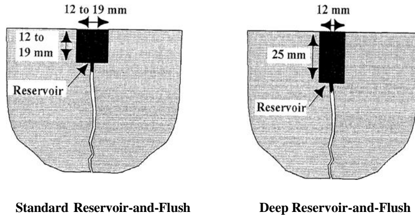
FIGURE 2 – RESERVOIR
